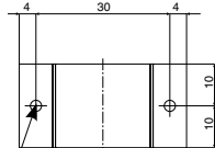
Hole for 2.9 x 9 self-threading screws
